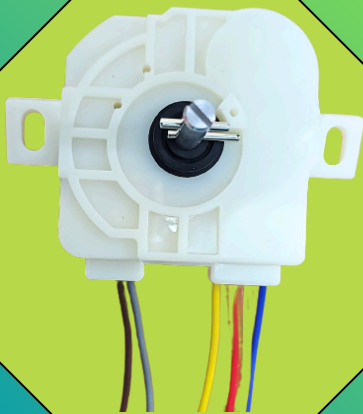
TW-003 CROSS-FITTING 6 WIRE
