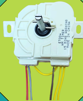
TW-004 CROSS-FITTING 5 WIRE
